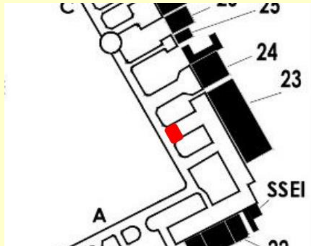
Figure 3. Enlarged chart of San Fernando Aerodrome, sector access road to hangar 23 closed (FROM DTHR 23 TO 470 M UNTIL HANGAR 23).
