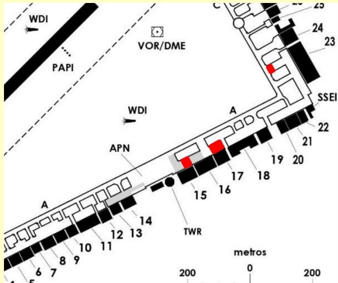
Figure 2. Enlarged chart of San Fernando Aerodrome, sector hangars 15 and 17 flexible-pavement aprons with restrictions for all aircraft, vehicles and persons operations.
